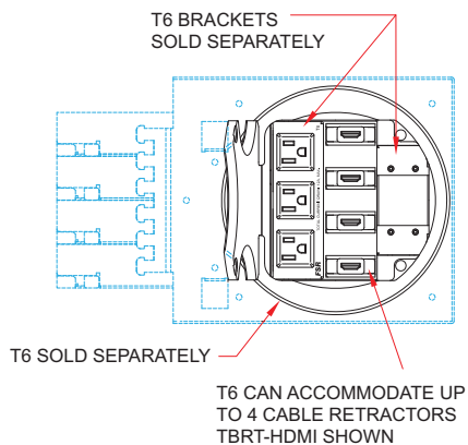
ASSEMBLED VIEW WITH CABLES EXTENDED
