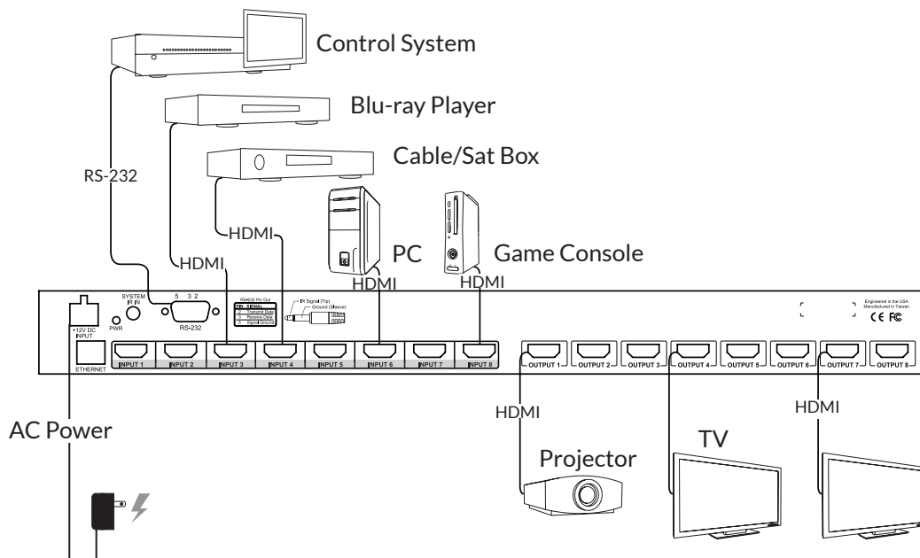
FIGURE 3: B-120-HDMATRIX-8x8 Installation
