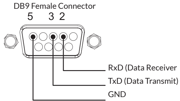
FIGURE 4: RS-232 (DB9) Pin Configurations
