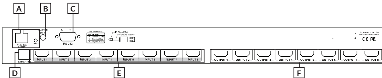
FIGURE 2: B-120-HDMATRIX-8x8 Switcher Layout (Rear View)
