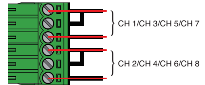
[Unbalanced cable]
