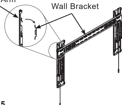
Figure 4 Mount Arm
